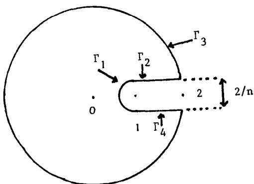
FIG. 2. The contour \Gamma used in the proof of Proposition 2.
