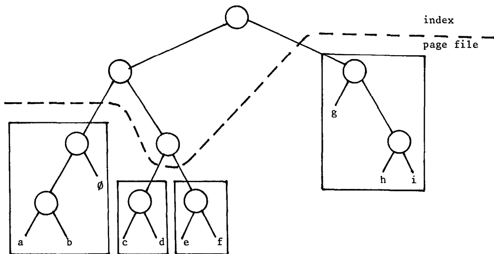
FIG. 4. The paged 2-d-trie corresponding to F = \{a, b, \dots, i\} with page capacity 3 when a = (00-, 00-) , b = (00-, 01-) , c = (00-, 10-) , d = (00-, 11-) , e = (01-, 10-) , f = (01-, 11-) , g = (1-, 0-) , h = (10-, 1-) , and i = (11-, 1-) .
