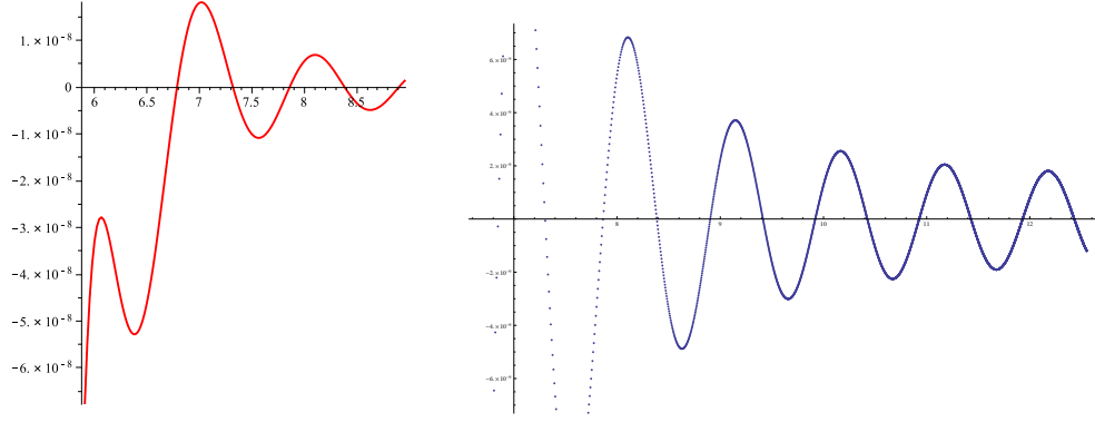
FIGURE 6. Left : The difference (PA_n - \Omega_6)2^{-n}n^{-g} against \log_2 n , where \Omega_6 is the six-term extension of (74), for n = 60, \dots, 500 ; the plot reveals about three periods of the oscillating component in the asymptotic expansion of PA_n . Right : The corresponding plot, for values up to n = 6000 . The diagrams confirm the presence of oscillations that, asymptotically, have amplitude of the order of 10^{-9} .
