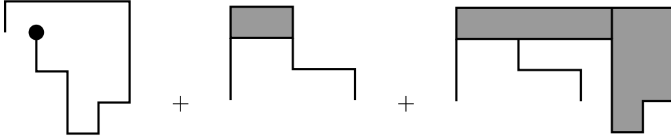
FIGURE 3. The decomposition used to construct 3-sided prudent polygons.
