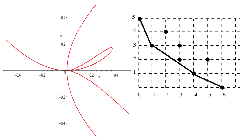
FIGURE 16. The real curve defined by the equation P = (y - x^2)(y^2 - x)(y^2 - x^3) - x^3y^3 near (0, 0) (left) and the corresponding Newton diagram (right).
