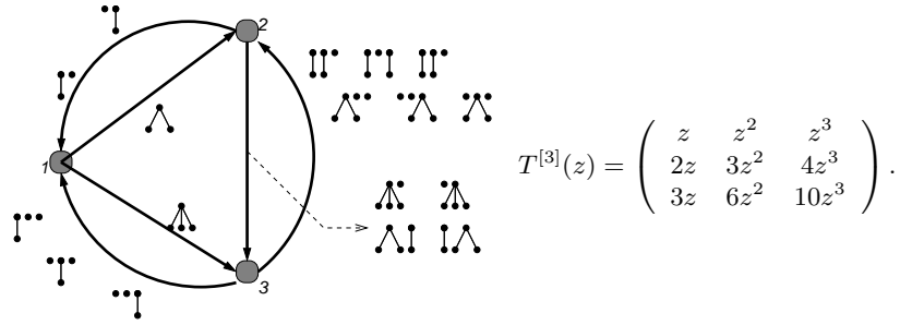
FIGURE 20. The sized graph corresponding to general plane trees of width at most 3 and the corresponding transfer matrix. (The transitions from a node to itself are omitted, for readability.)
