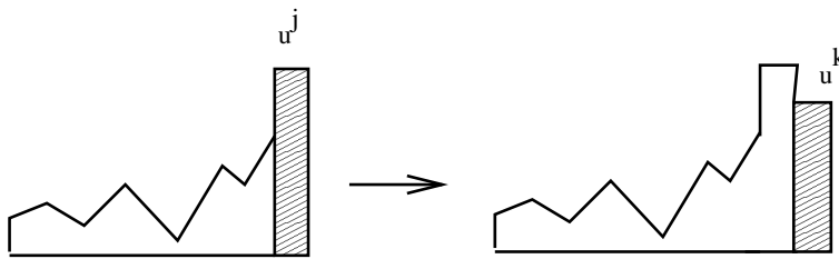
FIGURE 14. The technique of “adding a slice” for enumerating constrained compositions.
