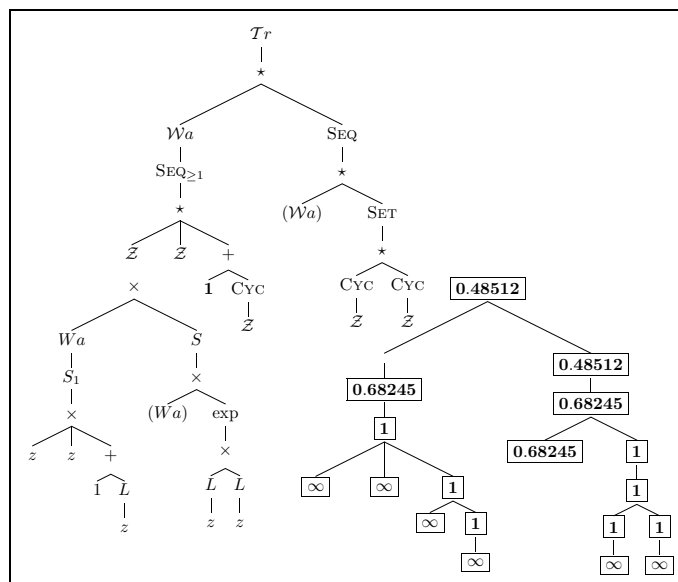
FIGURE 6. The inductive determination of the radius of convergence of the EGF of trains: (top) a hierarchical view of the specification of \mathcal{T}r ; (bottom left) the corresponding expression tree of the EGF Tr(z) ; (bottom right) the value of the radii for each subexpression of Tr(z) (with L(y) = \log(1 - y)^{-1} , S(y) = (1 - y)^{-1} , S_1(y) = yS(y) ).
