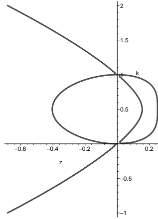
FIGURE 18. The algebraic curve associated to the generating function of supertrees of type K .
