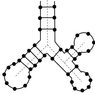
FIGURE 11. A simplified combinatorial model of RNA structures as considered by Waterman et al. [267, 423, 444].
